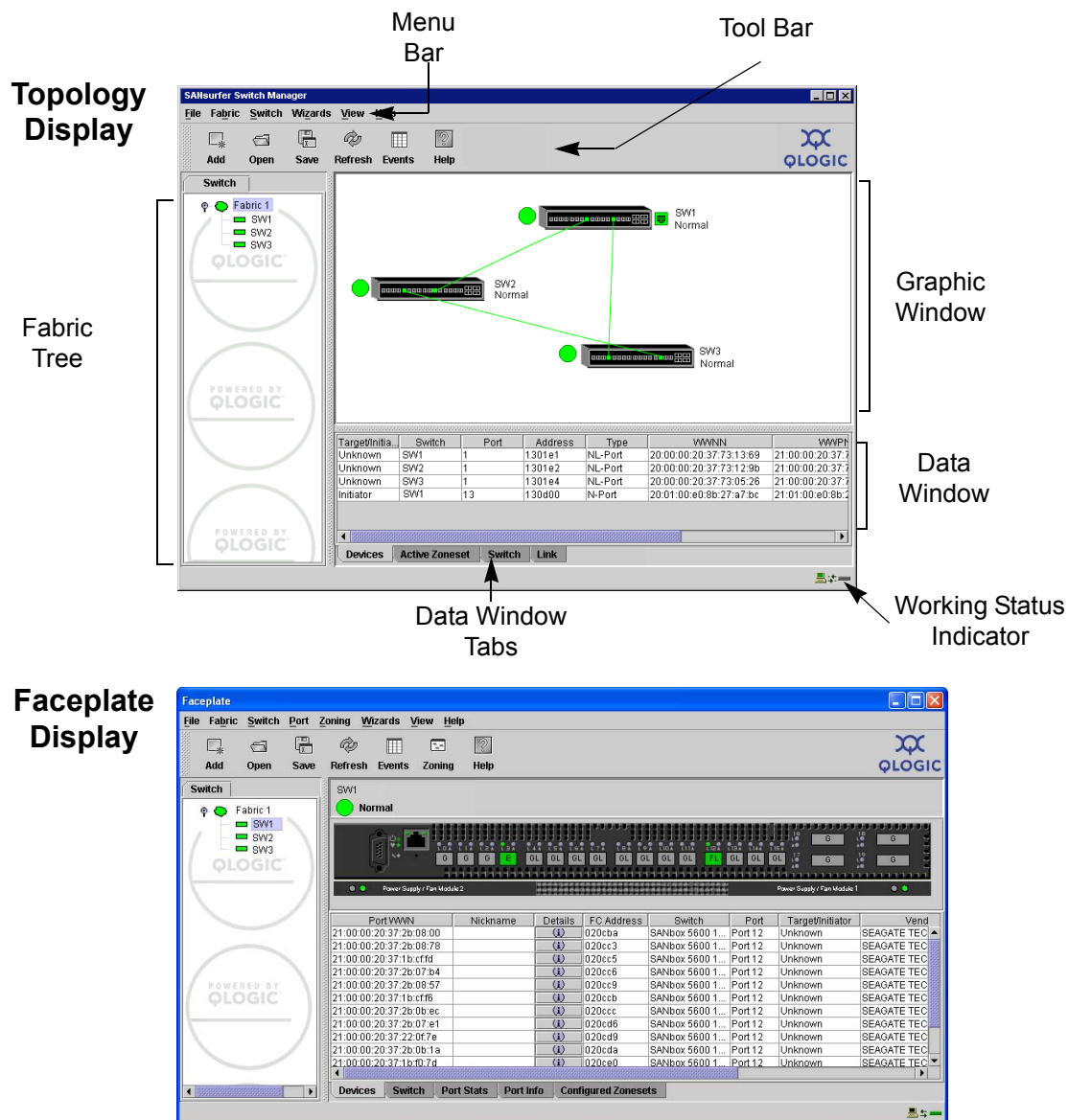
Figure 2-6. SANsurfer Switch Manager Display Elements
