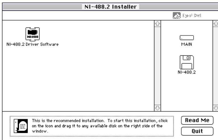
Figure 3-1. Installer Window
