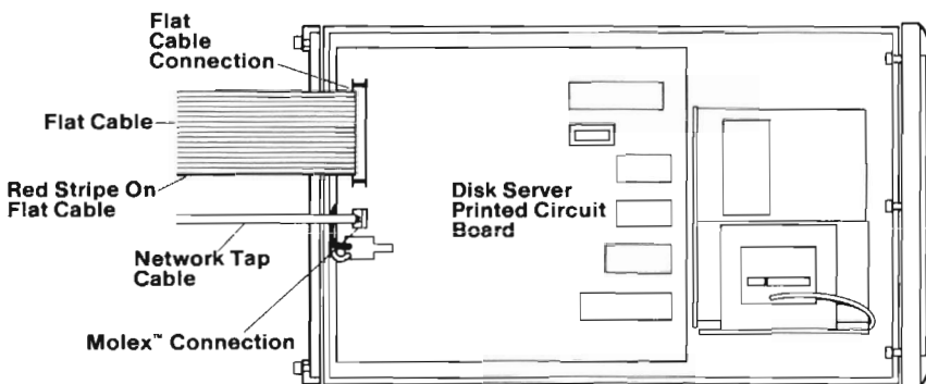
Flat Cable and Network Tap Connection
