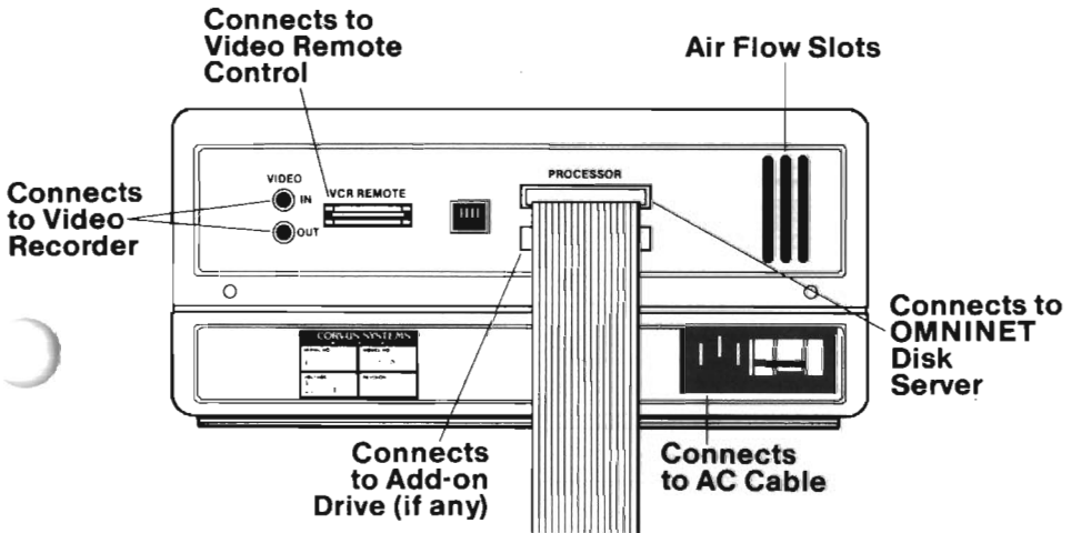
Back Panel of the Corvus Drive
