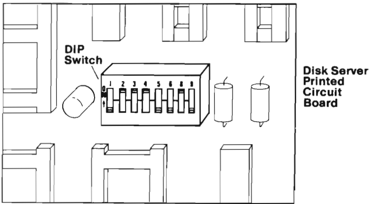
DIP Switch for Setting the Device Address
