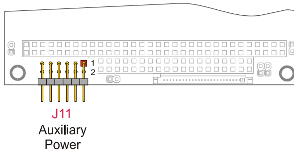
Figure 1. J11 Connector layout
