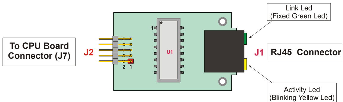
Figure 3. Ethernet Adapter
